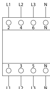
RCD ETI Type B in 3-phase system U_n = 240/415\text{V}
