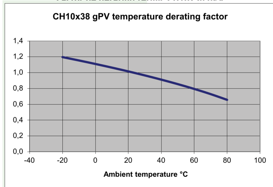
Factor de derating termic CH10x38 gPV
