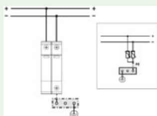
ETITEC S C-PV 75...1000/20 V-Konfiguration
