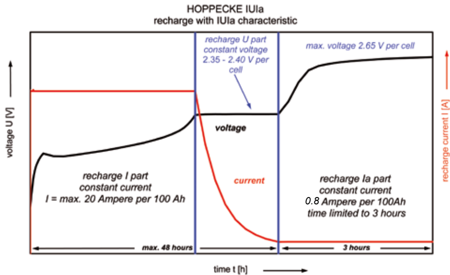
Fig. 9-2: IUa characteristic
